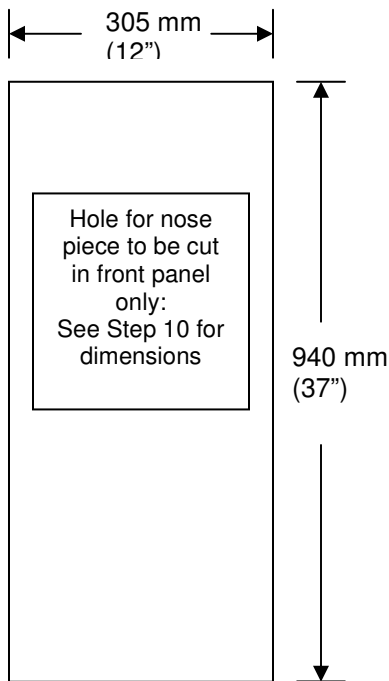
Exterior Back and Front panels (2 pieces)
