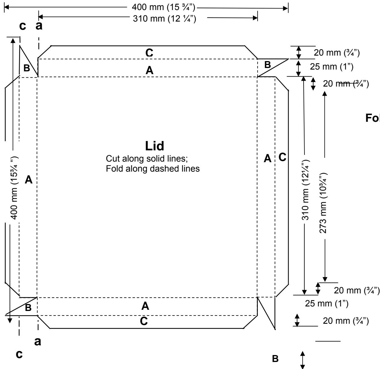
Figure 2 Filter Lid
